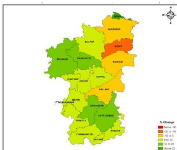
Figure 22: Change in precipitation by 2021-50, for the rabi season in the Krishna basin (A1B) 2
